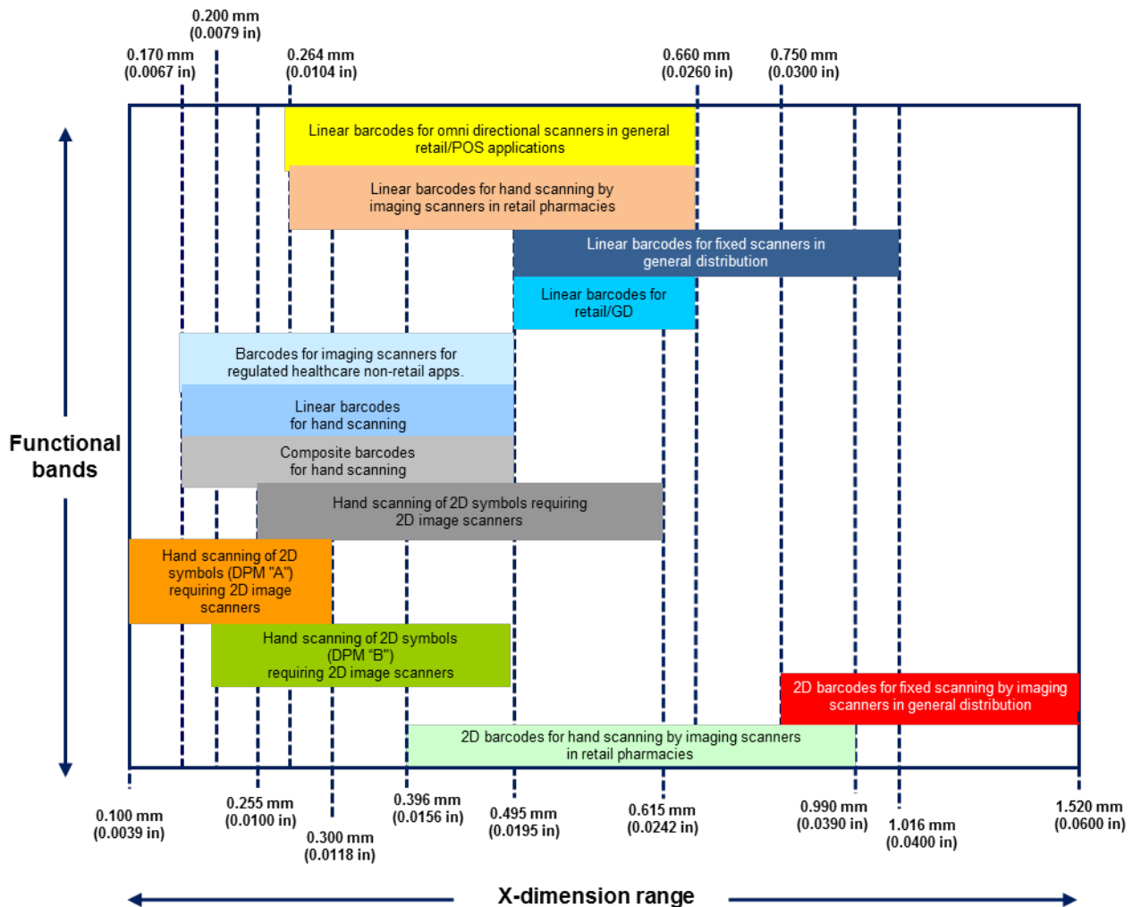
Figure 5.9.2.6-1. GS1 scanner functional operative bands
