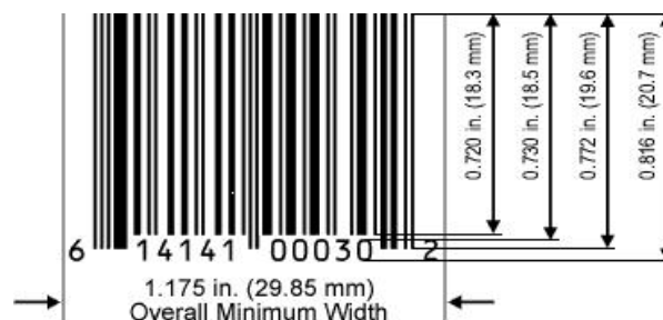
Figure 5.9.6.3-1. EAN/UPC symbol shown with minimum height and overall width dimensions for magnifications of 75 percent to 80 percent
