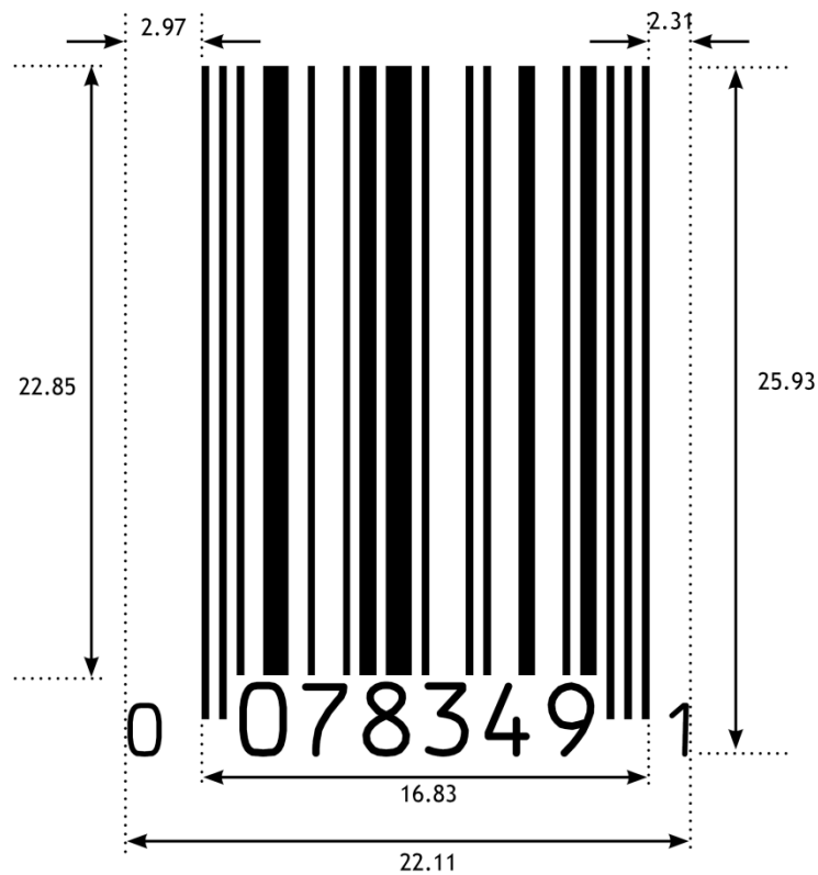
Figure 5.2.6.6-4. UPC-E barcode
