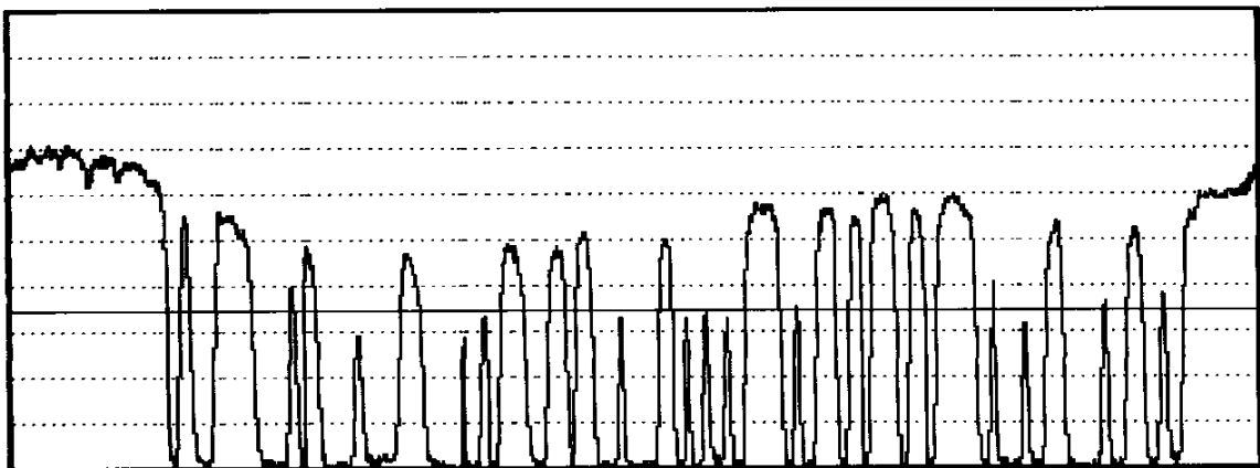
Figure 5.9.5.12-2. Scan Reflectance Profile with narrow space profiles
