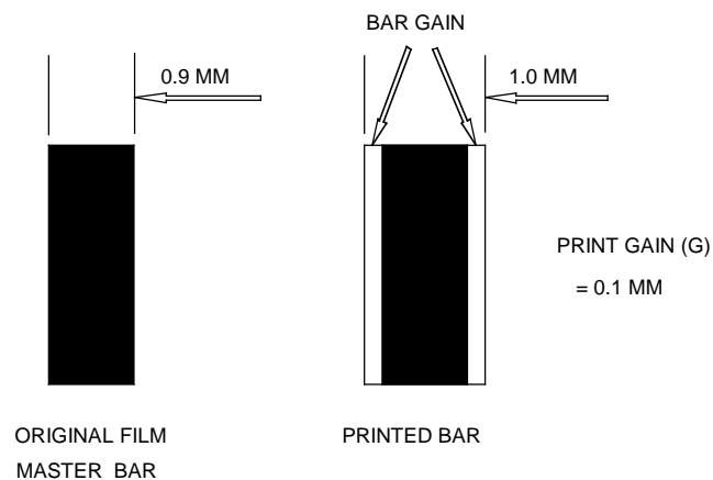
Figure 5.9.4.2.1-1. Example of bar width adjustment
