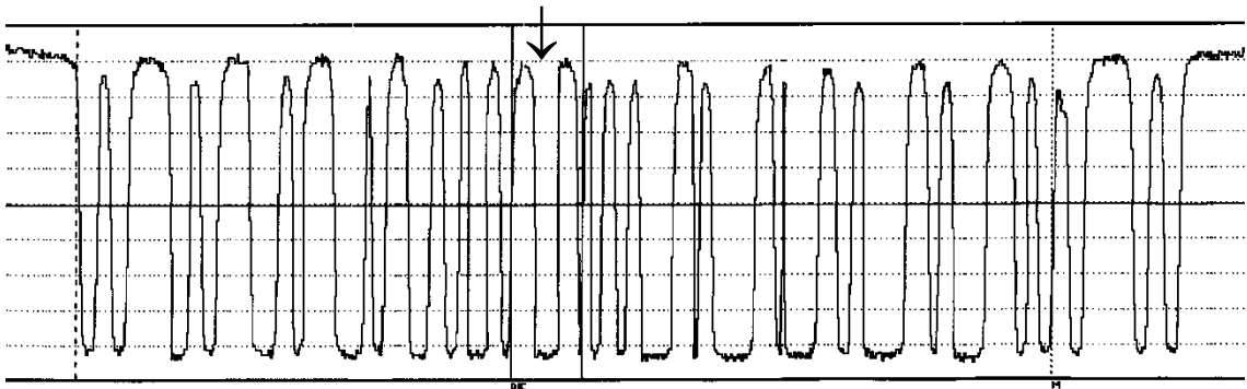
Figure 5.9.5.12-4. Scan Reflectance Profile of symbol with low decodability character
